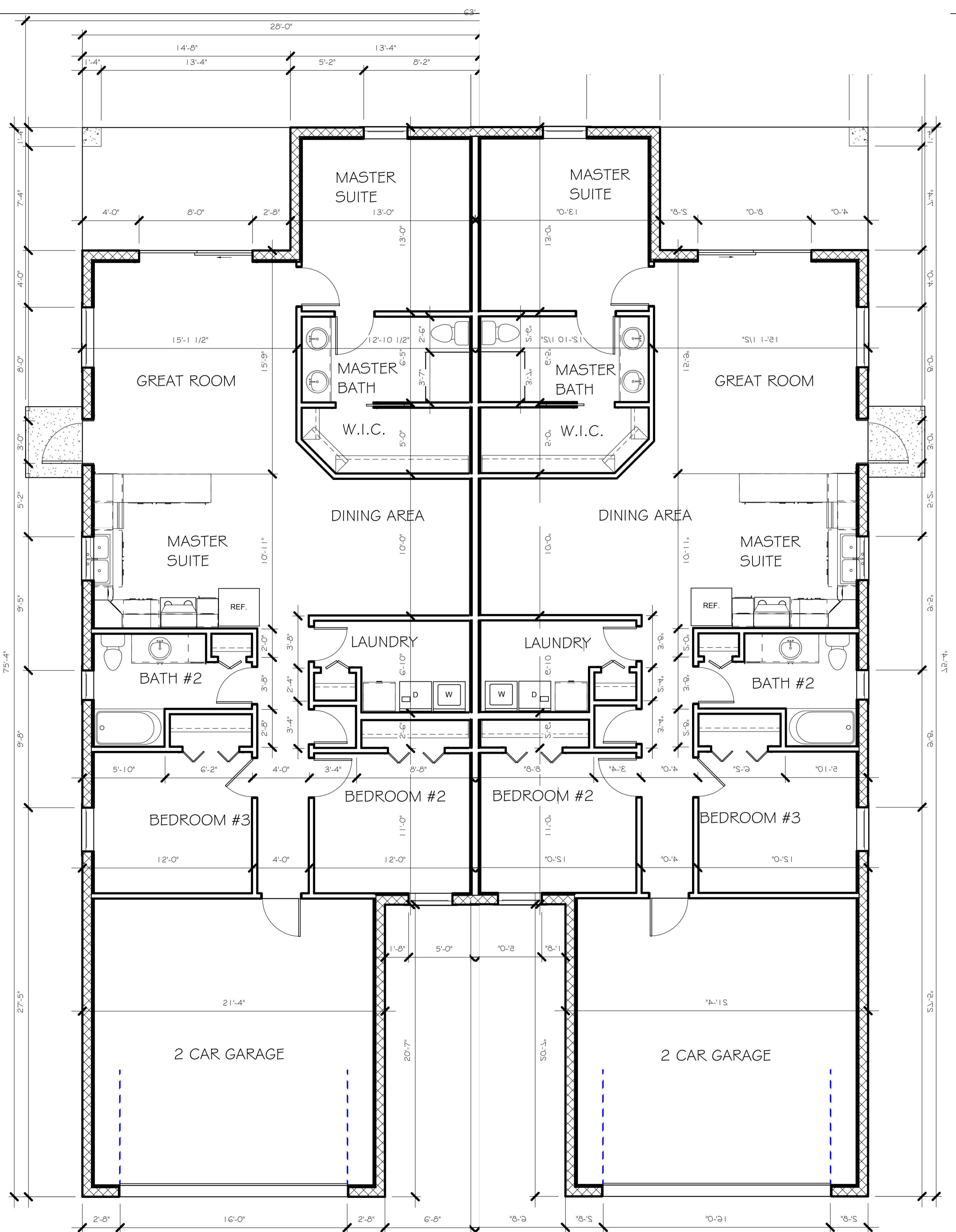
FLOOR PLAN
